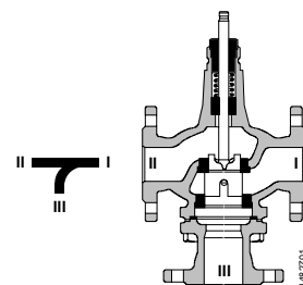
DN 40...150
